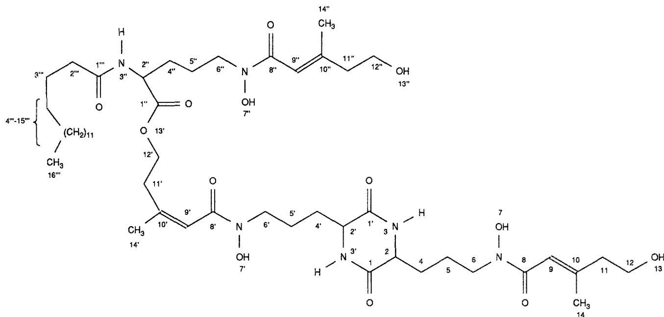
Fig. 2. Structure of desferripalmitoylcoprogen
